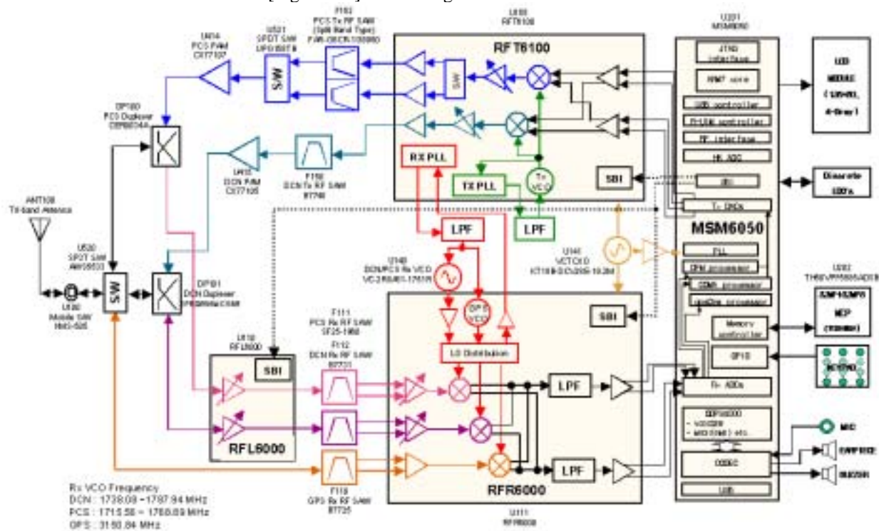
[Figure 1-1] Block Diagram of LG-TM250
